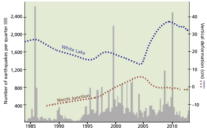
Number of earthquakes in the park each calendar quarter and vertical movement recorded at White Lake and Norris Junction.
