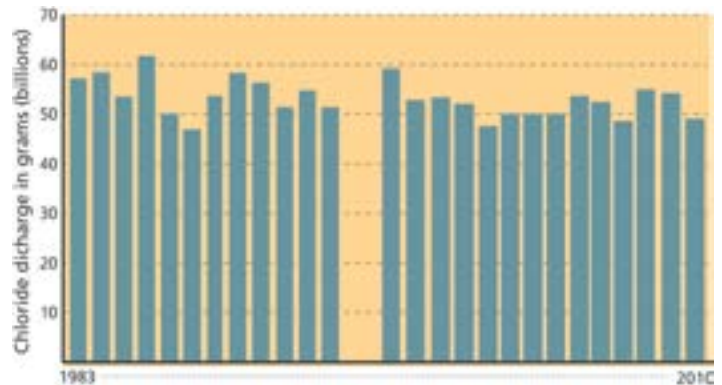
Total annual chloride discharge from Yellowstone's major rivers from 1983 to 2010. (No samples collected in 1995 and 1996.)
