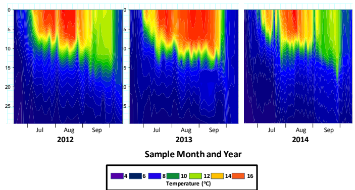
Figure 25. Yellowstone Lake isopleths showing seasonal and annual variation in water temperature throughout the water column, 2012-2014. Only upper 30 meters are shown (y-axis) for better resolution of surface water temperatures.
