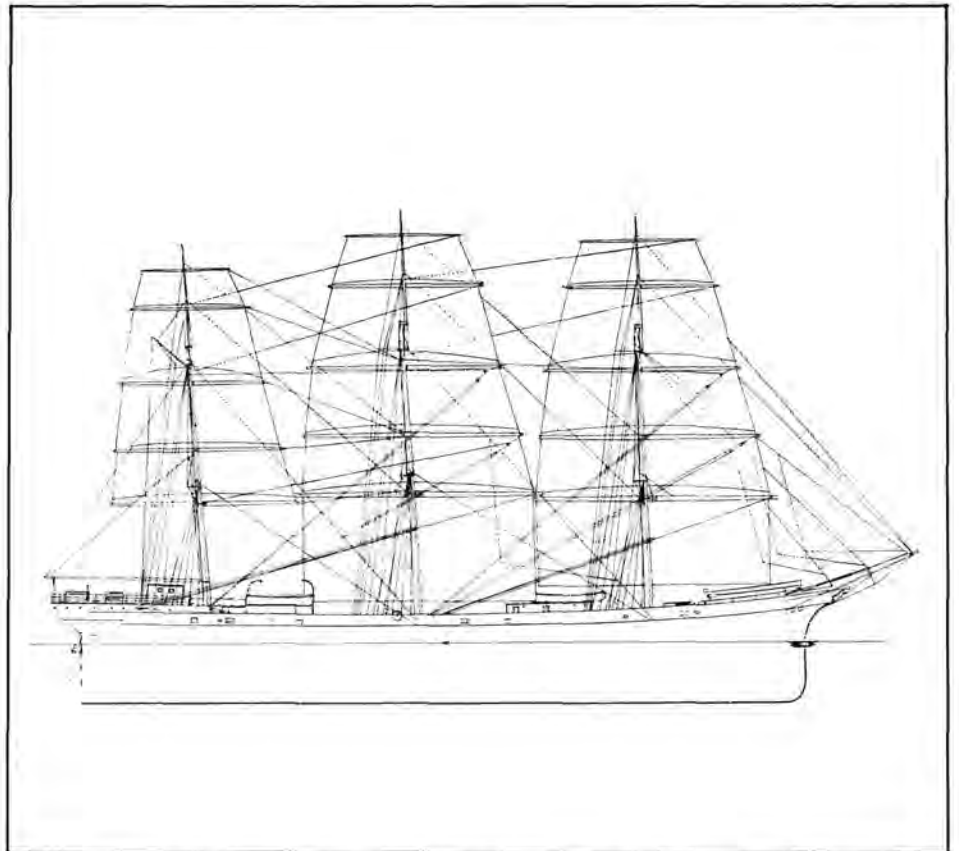
Balclutha (Star of Alaska), traced from an original Rigging Plan by Captain C. A. Halvorson 1909..F. W. Shaw, August 1944.
