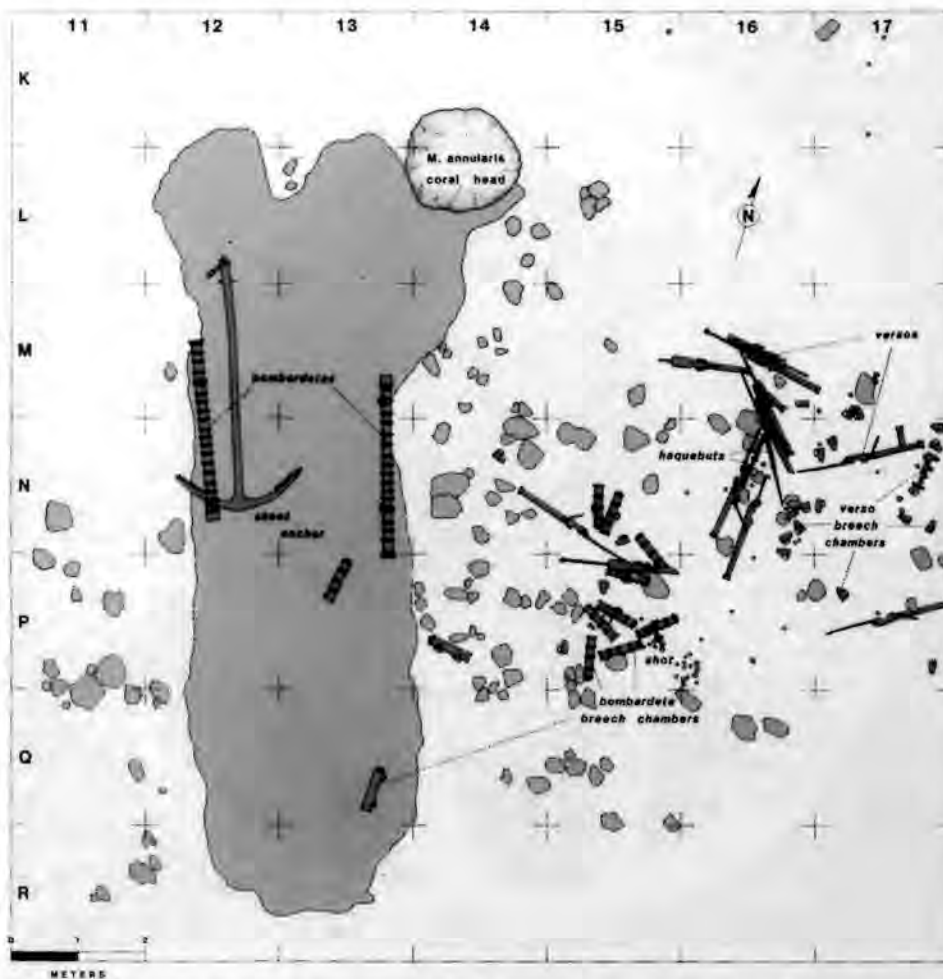
Plan showing wrought iron ordnance on the Molasses Reef Wreck, an early 16th century shipwreck site in the Turks and Caicos Islands. This wreck, first thought to be Columbus' Pinta , was heavily armed and carried a cargo of cannon when lost.
