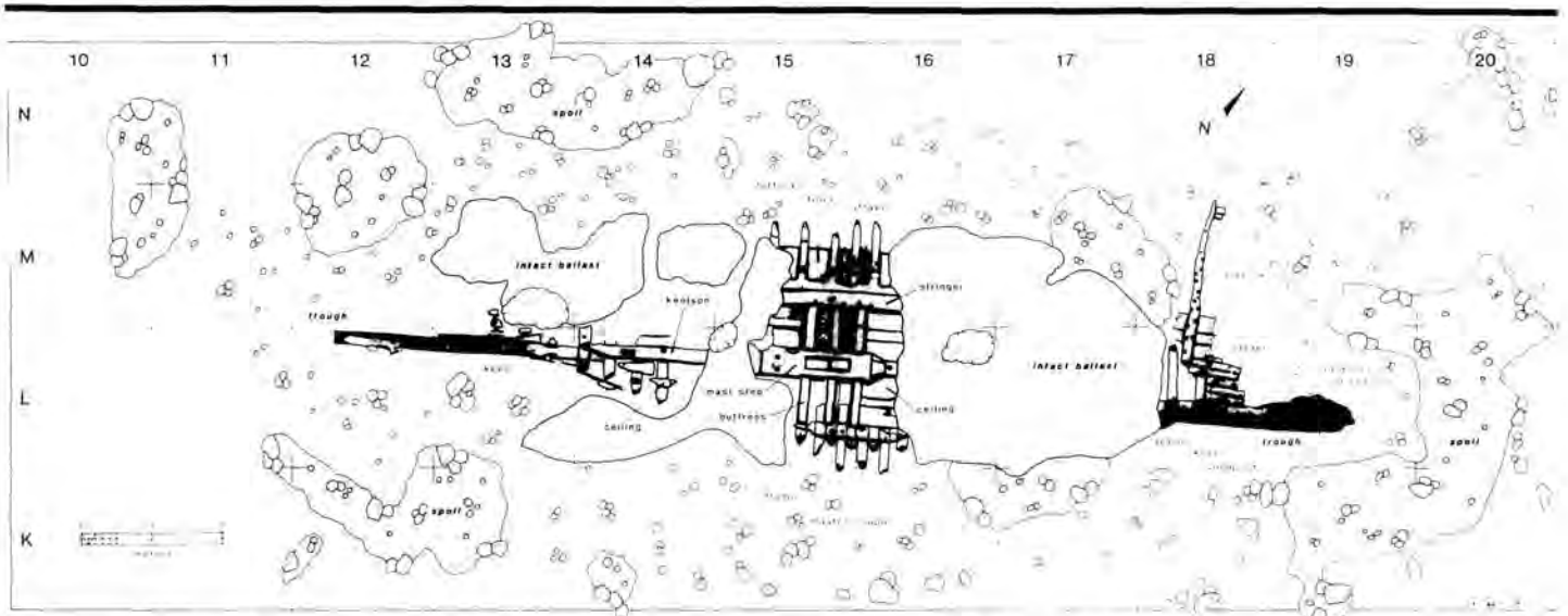
Excavation plan for the Highborn Cay Wreck. Located in the Exuma Island chain in the Bahamas, this wreck has the best preserved hull remains of any early 16th century ship yet discovered in the Caribbean.
