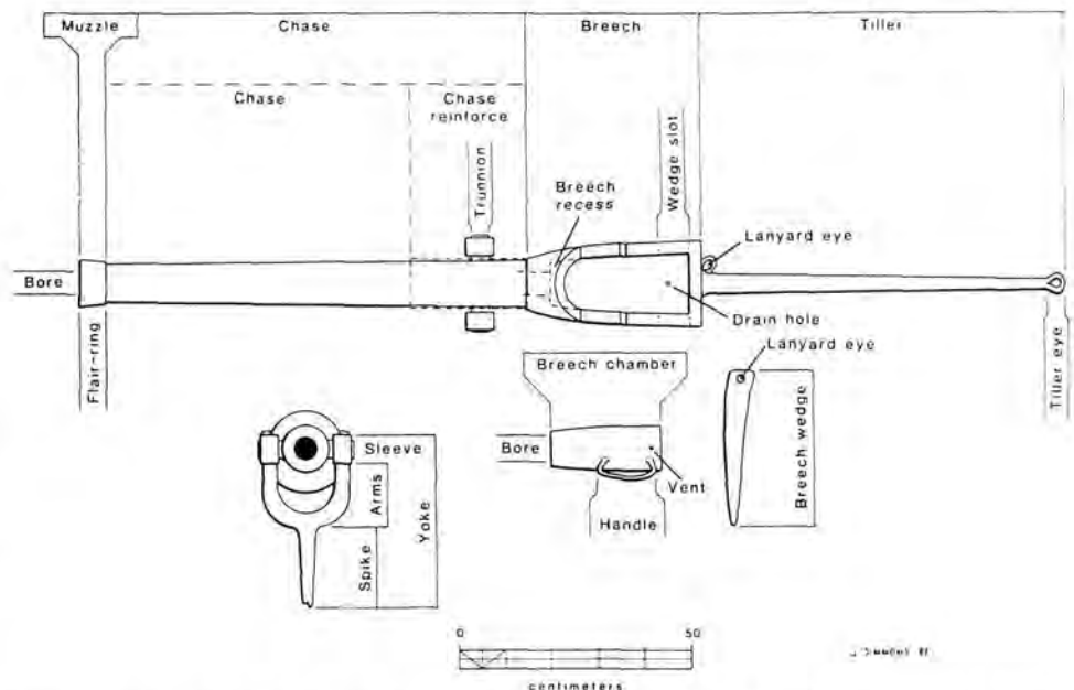
Reconstruction drawing of a Spanish verso from the Molasses Reef Wreck, illustrating a typical shipboard weapon from the age of exploration.
