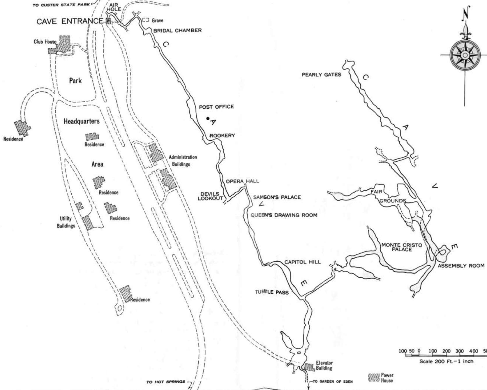
UNDERGROUND SURVEY, WIND CAVE NATIONAL PARK
