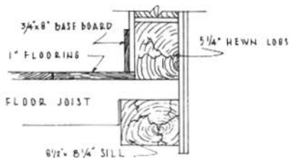
TYPICAL WALL SECTION SCALE: 1 1/2" = 1'-0"
