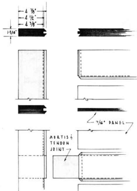
JOINING DETAILS SCALE 3" = 1'-0"
