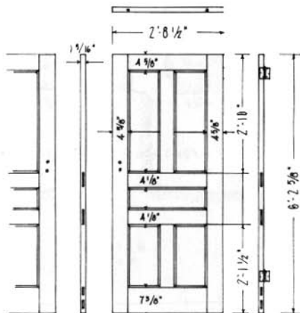
ELEVATIONS SCALE 3/4" = 1'-0"
