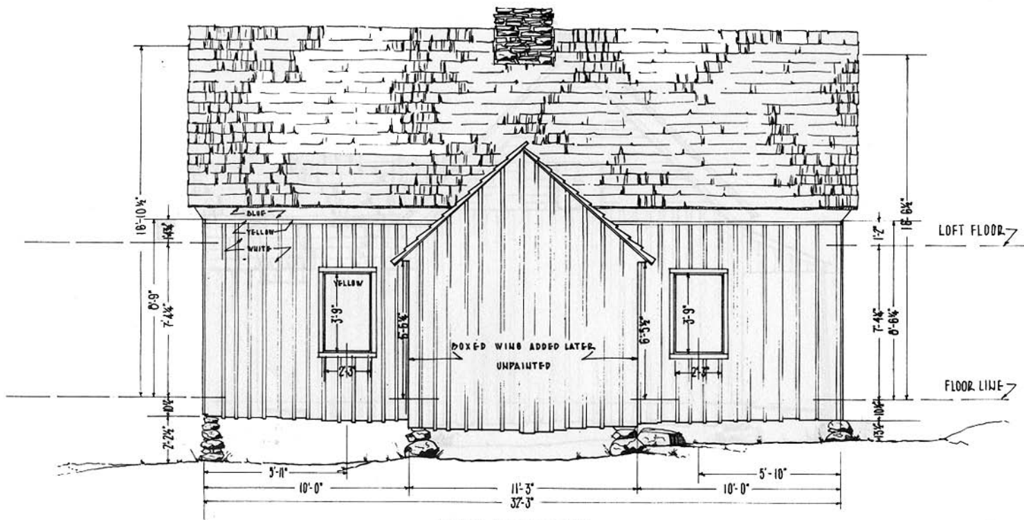
WEST ELEVATION
