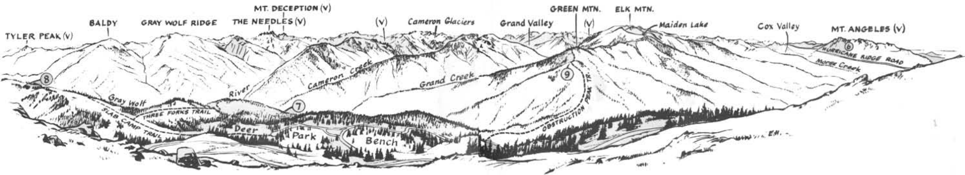
fig. 4. Panorama looking south from Blue Mountain (V means volcanic rock)
