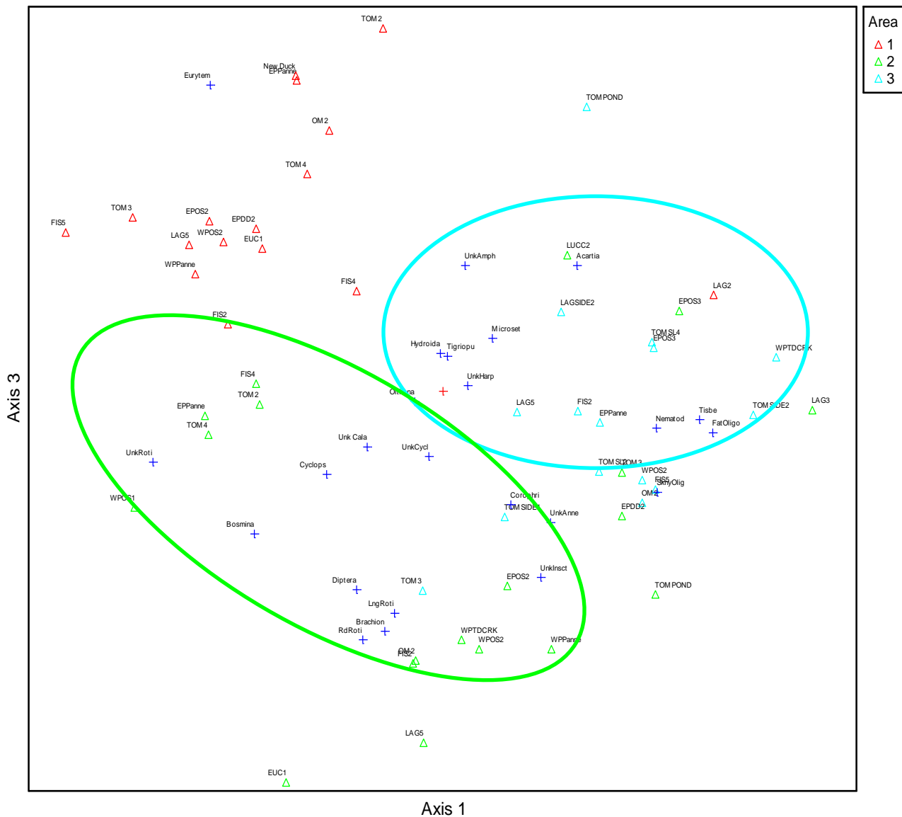
Figure 2. Statistical ordination of zooplankton species assemblages using Non-Metric Multi-Dimensional Scaling (NMDS) between different treatment periods in the Project Area. Pre-Restoration sites (labeled "1") separate from Passive Restoration sites (labeled "2") and Full Restoration sites (labeled "3").
