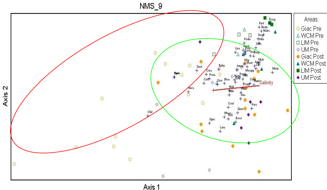
Figure 6. Two-dimensional (2D) ordination of Non-metric Multidimensional Scaling (NMS) coordinates. This graphic includes a joint plot of salinity, with a radiating line indicating the general strength and direction of correlation. Individual species are labeled and marked by blue crosshairs. Individual stations are coded by color and shape according to site. Circles correspond to Giacomini Wetland sites pre- and post-restoration.
