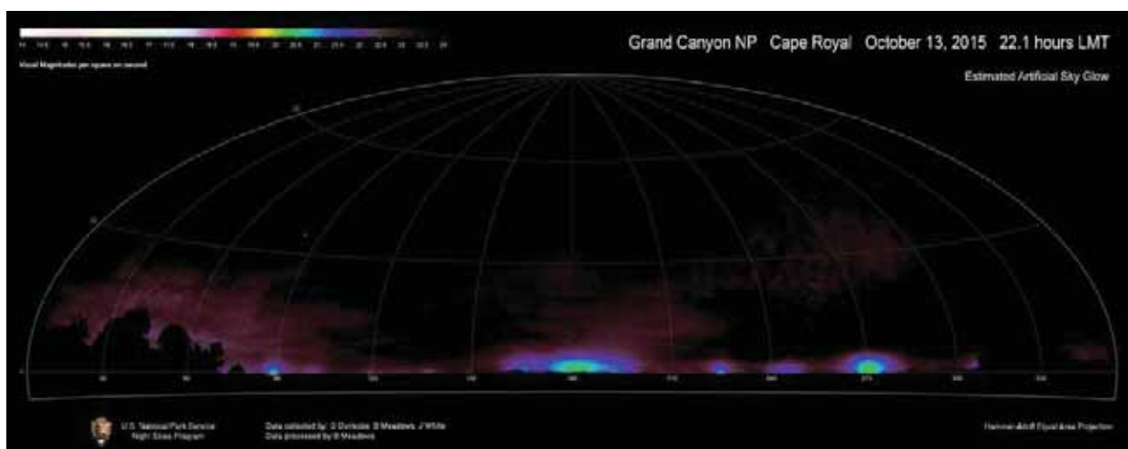
Figure 19. Estimated anthropogenic sky glow after subtraction of the natural sky model.
