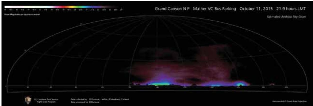
Figure 13. Estimated anthropogenic sky glow after subtraction of the natural sky model.
