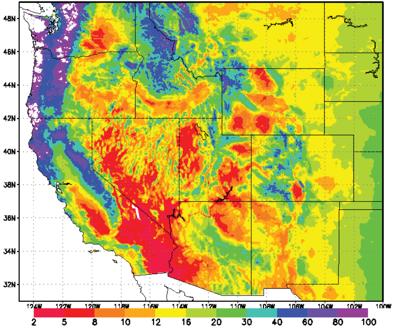
Figure 1. Average annual precipitation in inches as measured by the PRISM satellite. Data from the Western Regional Climate Center: http://www.wrcc.dri.edu/images/west.gif . Grand Canyon National Park is located in north-northwest Arizona with the inner canyon visible in the image as the thin strip of red running east-west.
