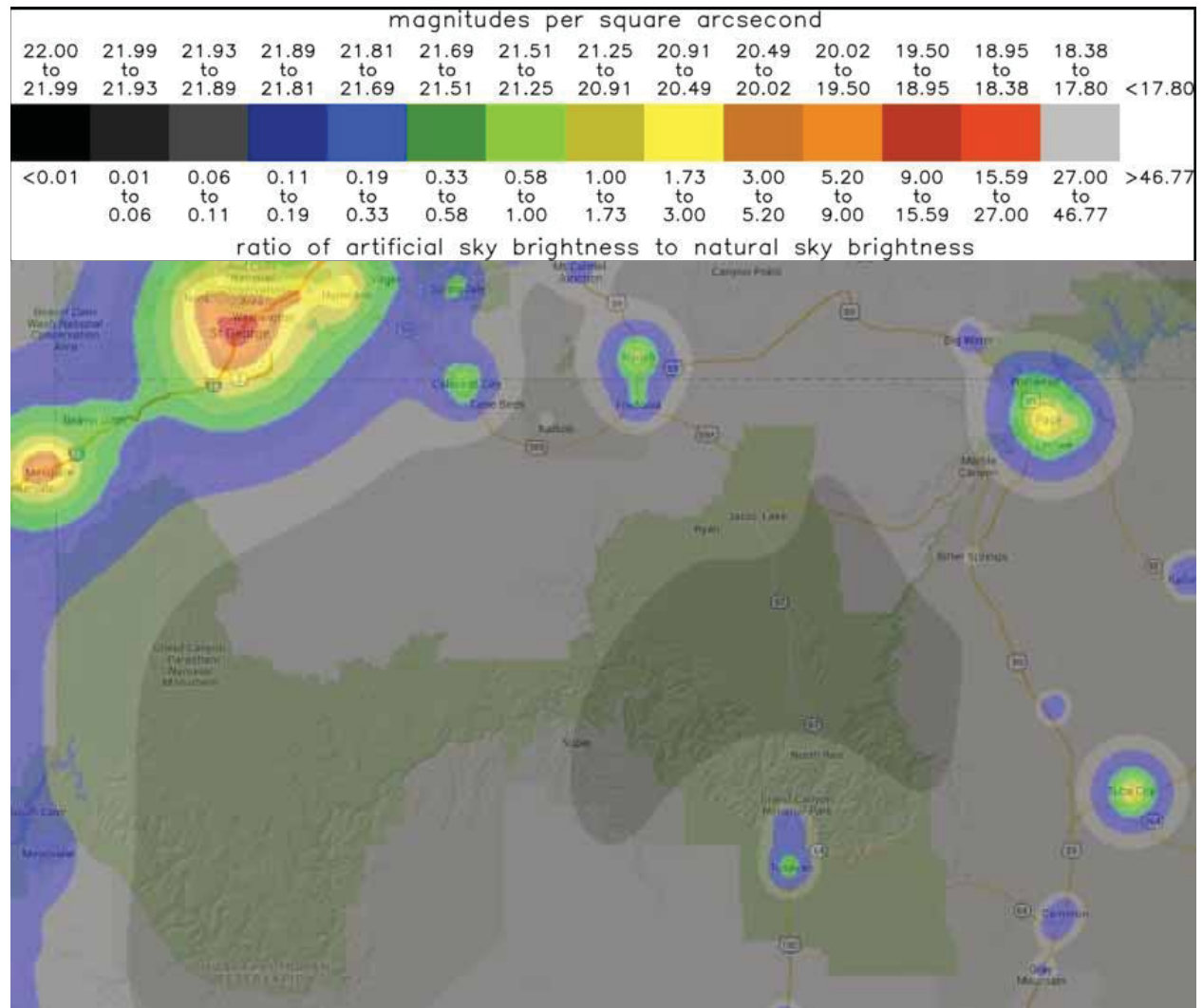
Figure 6. Ratio of artificial sky brightness to natural sky brightness and magnitudes per square arcsecond from David Lorenz's 2006 Light Pollution Atlas.
